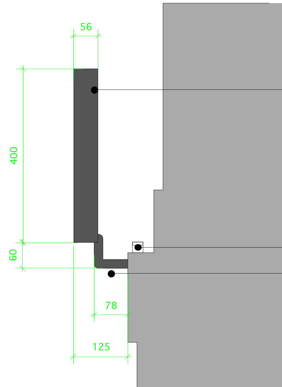
D2 - TYPICAL LETTERING DETAIL - MAIN SIGNAGE, FRONT AND SIDE ELEVATION 1:5 @ A1
