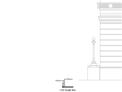
South West Elevation (Scale 1:50)
