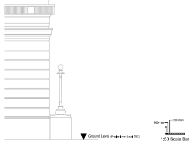
South East Elevation (Scale 1:50)
