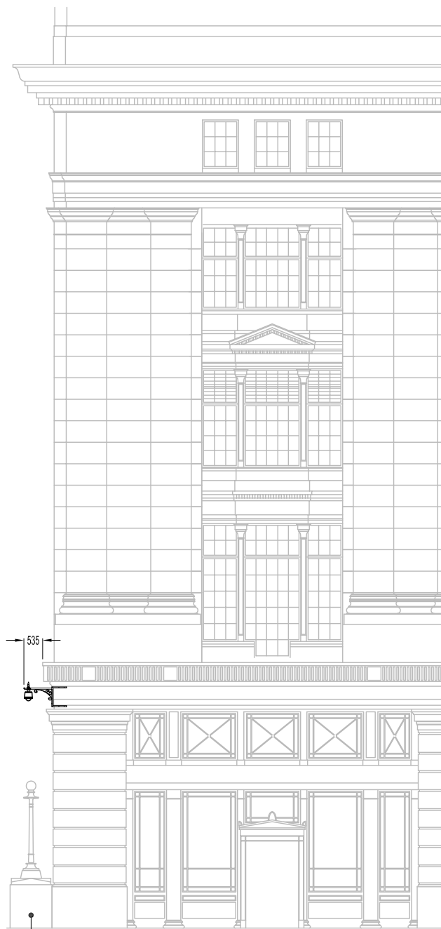
North East Elevation (Scale 1:50)
