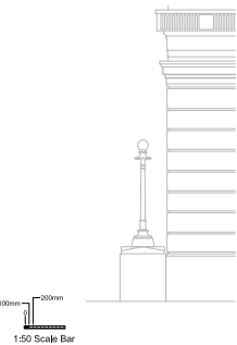
North East Elevation (Scale 1:50)
