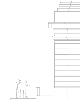
South East Elevation (Scale 1:50)
