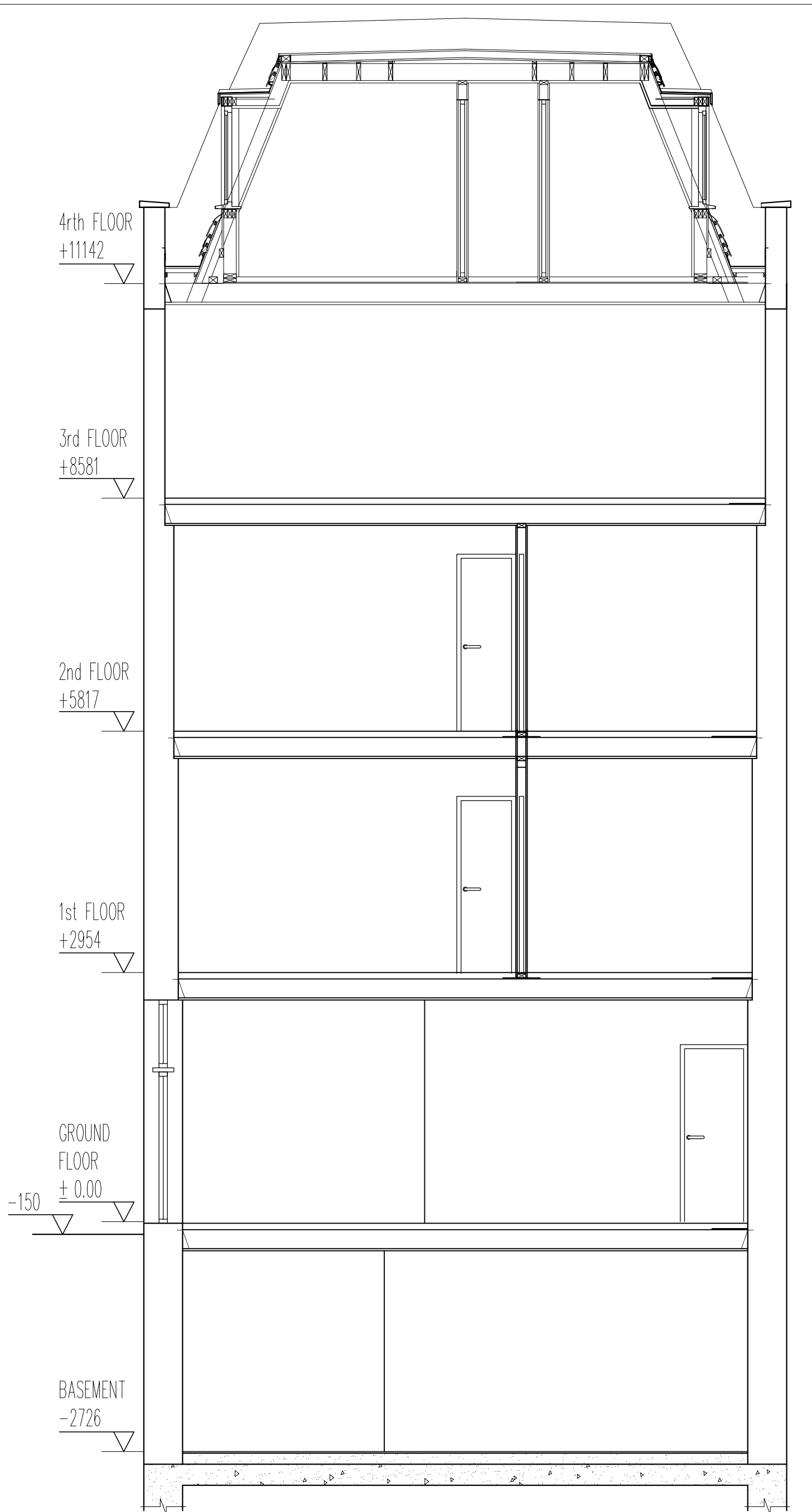
Section BB as Proposed
