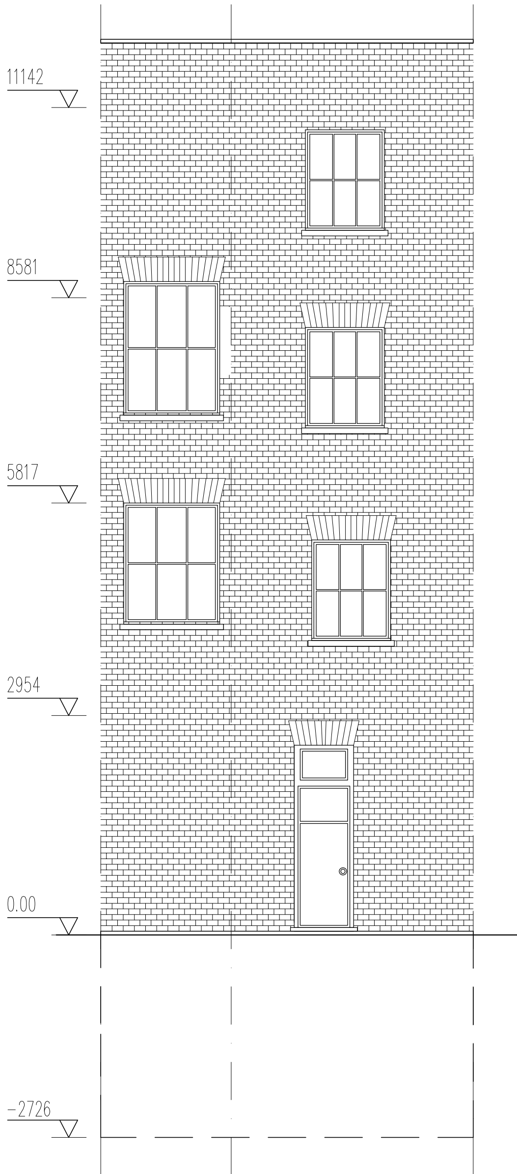
Rear Elevation as Existing
