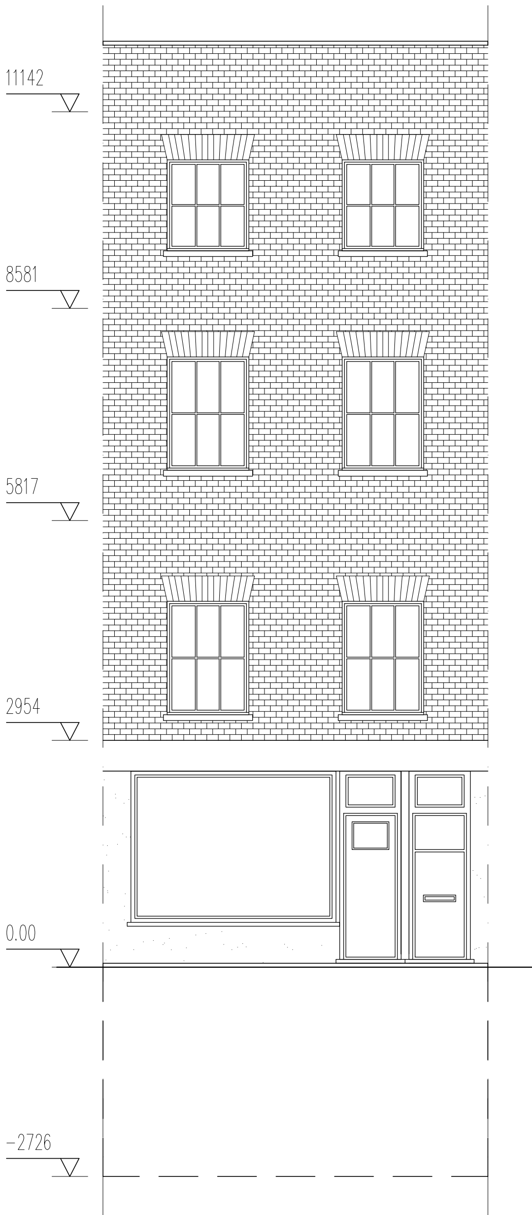
Front Elevation as Existing
