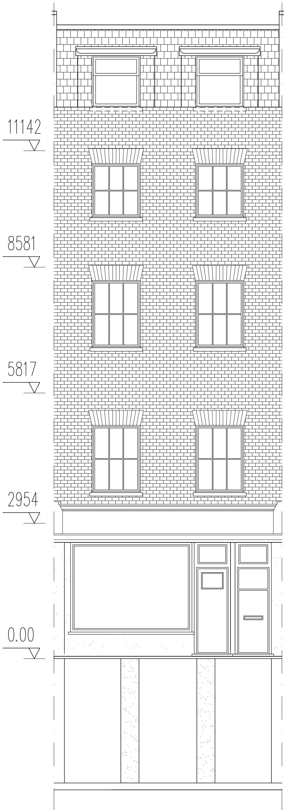
Front Elevation as Proposed Showing Lightwell
