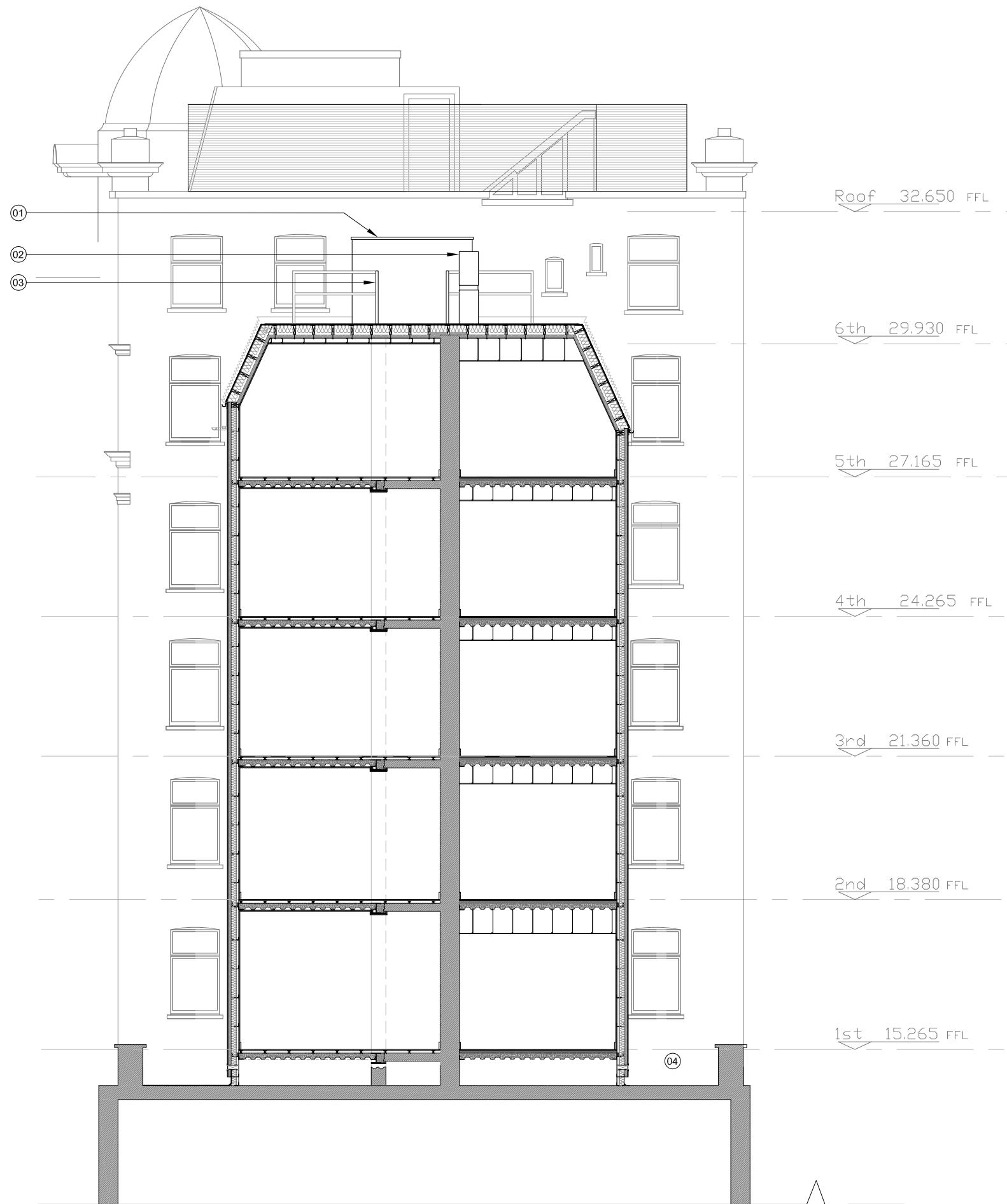
01 Section Through Infill, Existing Scale 1:100 @ A3
