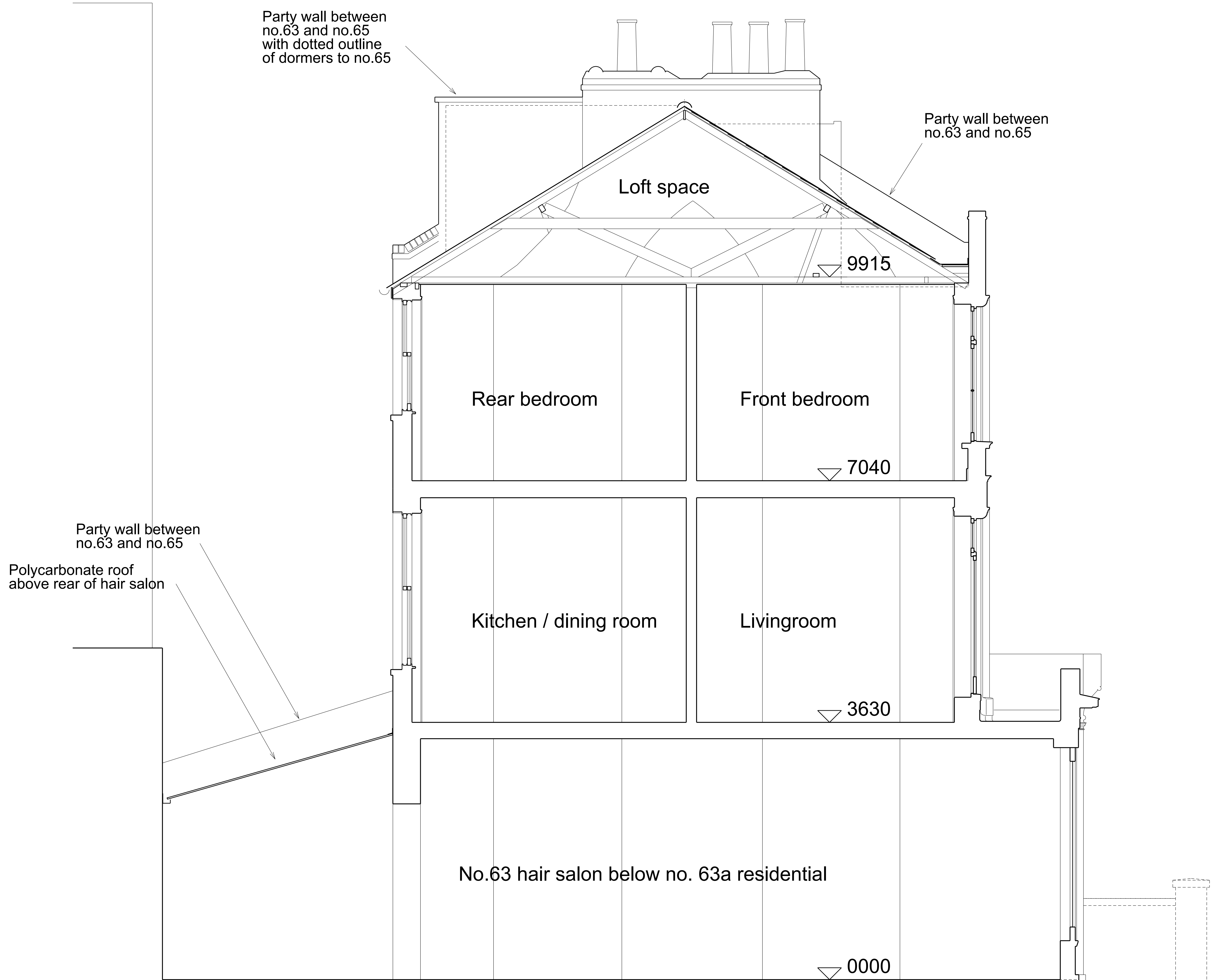
SECTION - AA - EXISTING
