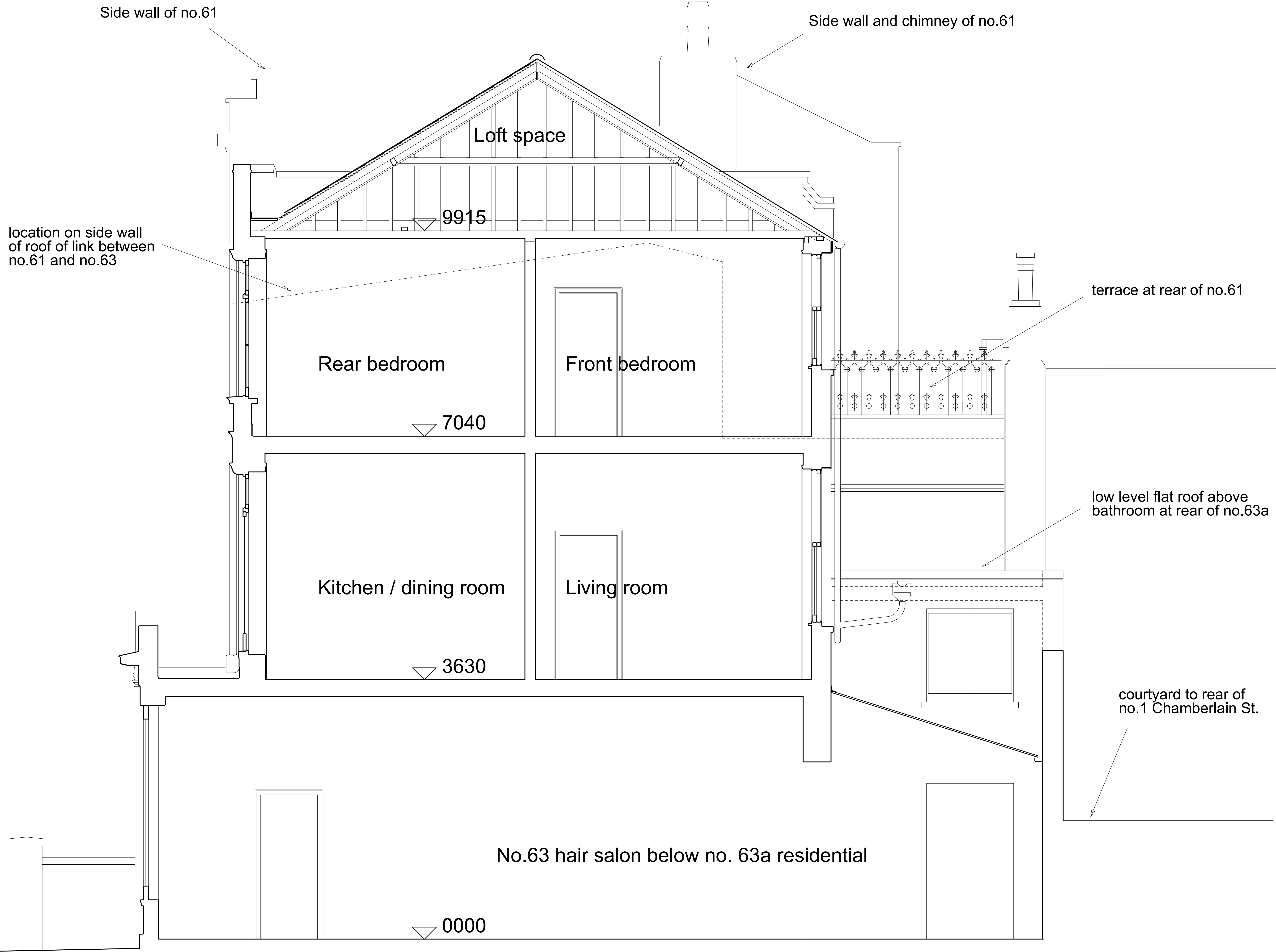
SECTION - BB - EXISTING
