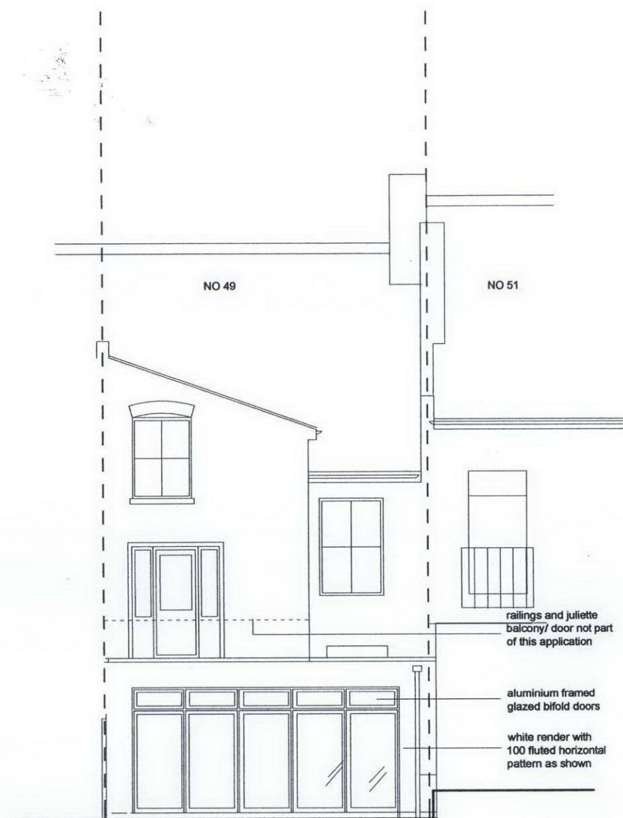
REAR ELEVATION 1 : 100
