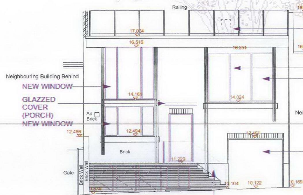
FRONT ELEVATION
