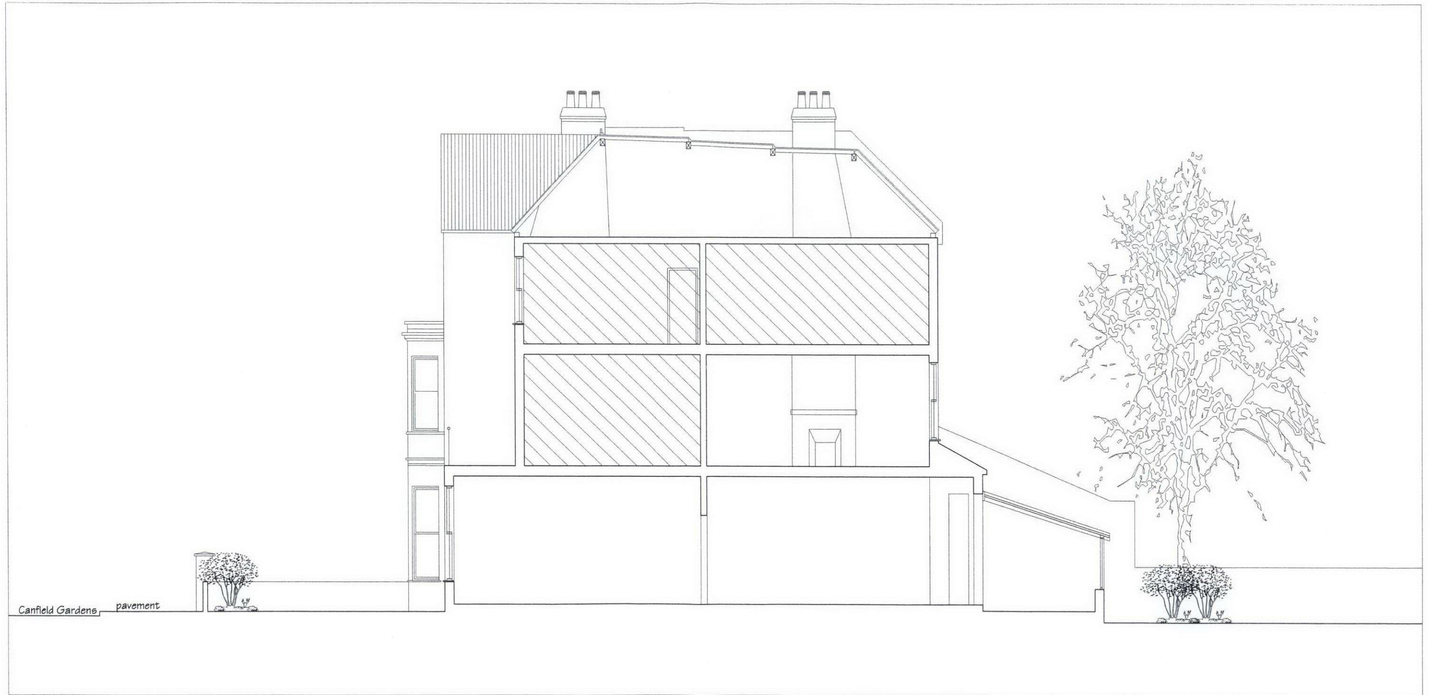
Cross Section A-A as Existing Scale 1:100 @A3
