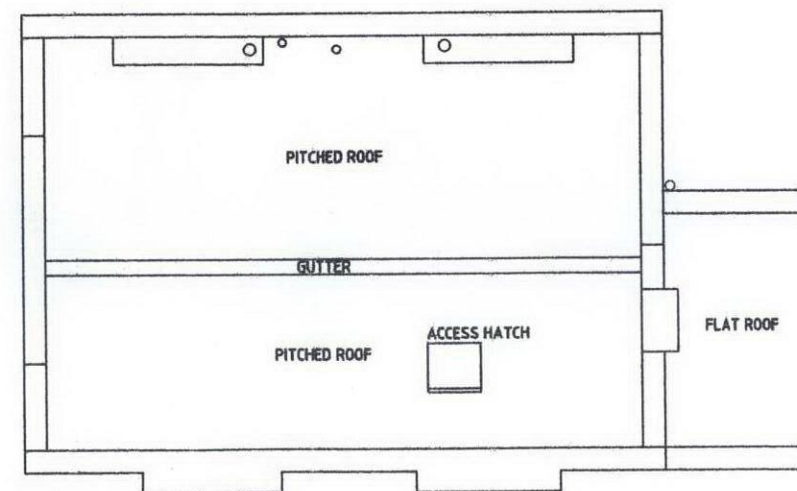
ROOF PLAN
