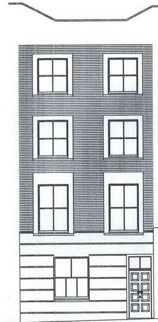
FRONT ELEVATION
