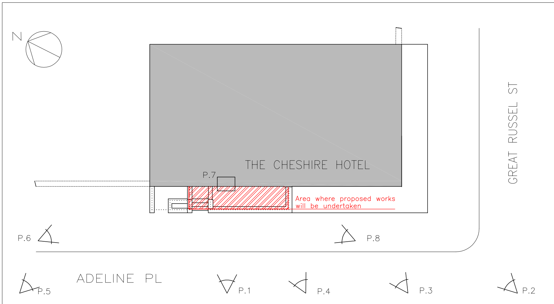
PHOTOGRAPHS REFERENCE PLAN SCALE 1:150 PHOTOGRAPHS: 22-10-2012
