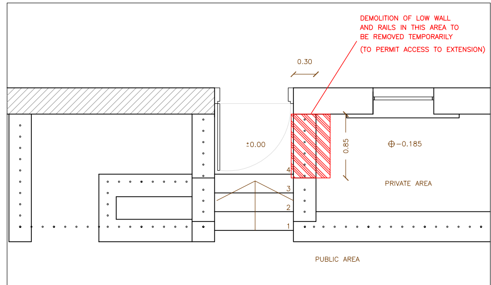
DEMOLITION PLAN SCALE 1:50 MEASURES IN METERS
