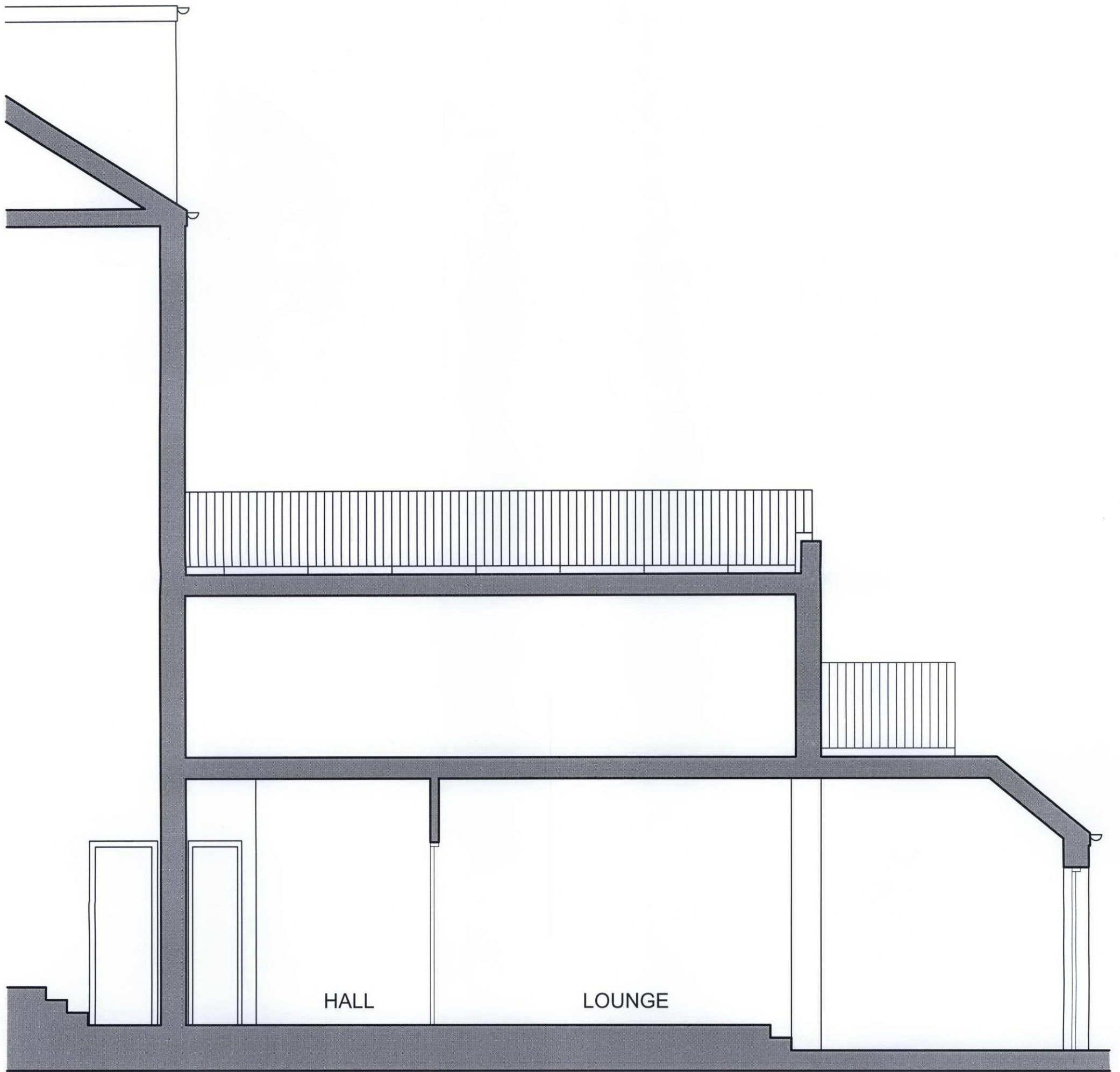
PROPOSED SECTION THROUGH OUTRIGGER AND EXTENSION
