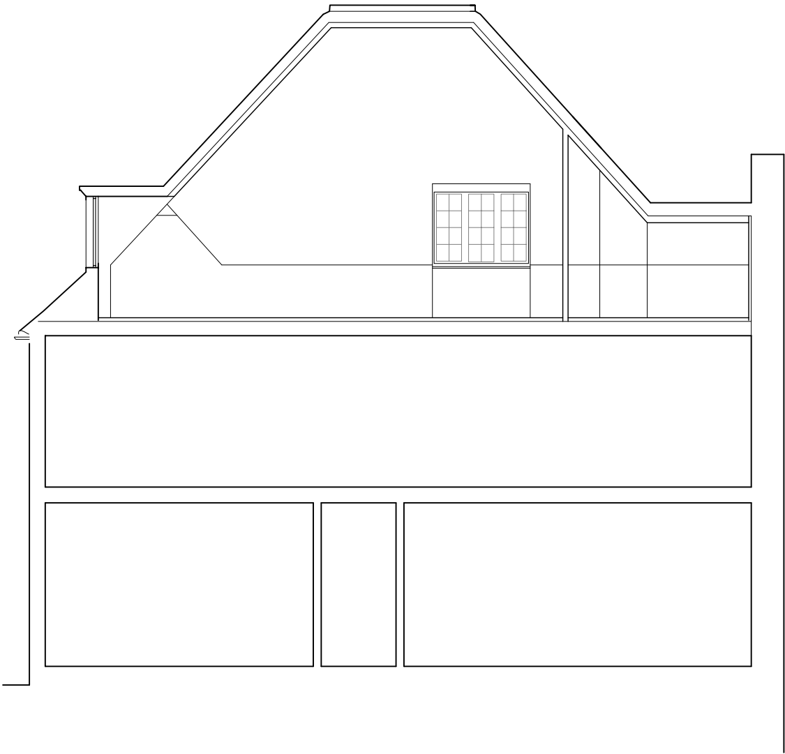
1 PROPOSED LONG SECTION 1 : 100
