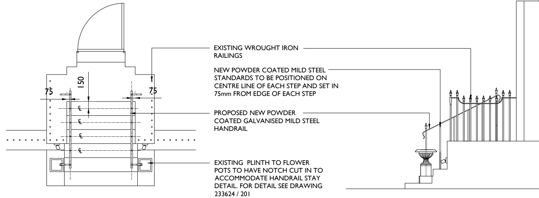
1 200 PLAN OF STEPS AS PROPOSED 1:50@A3
