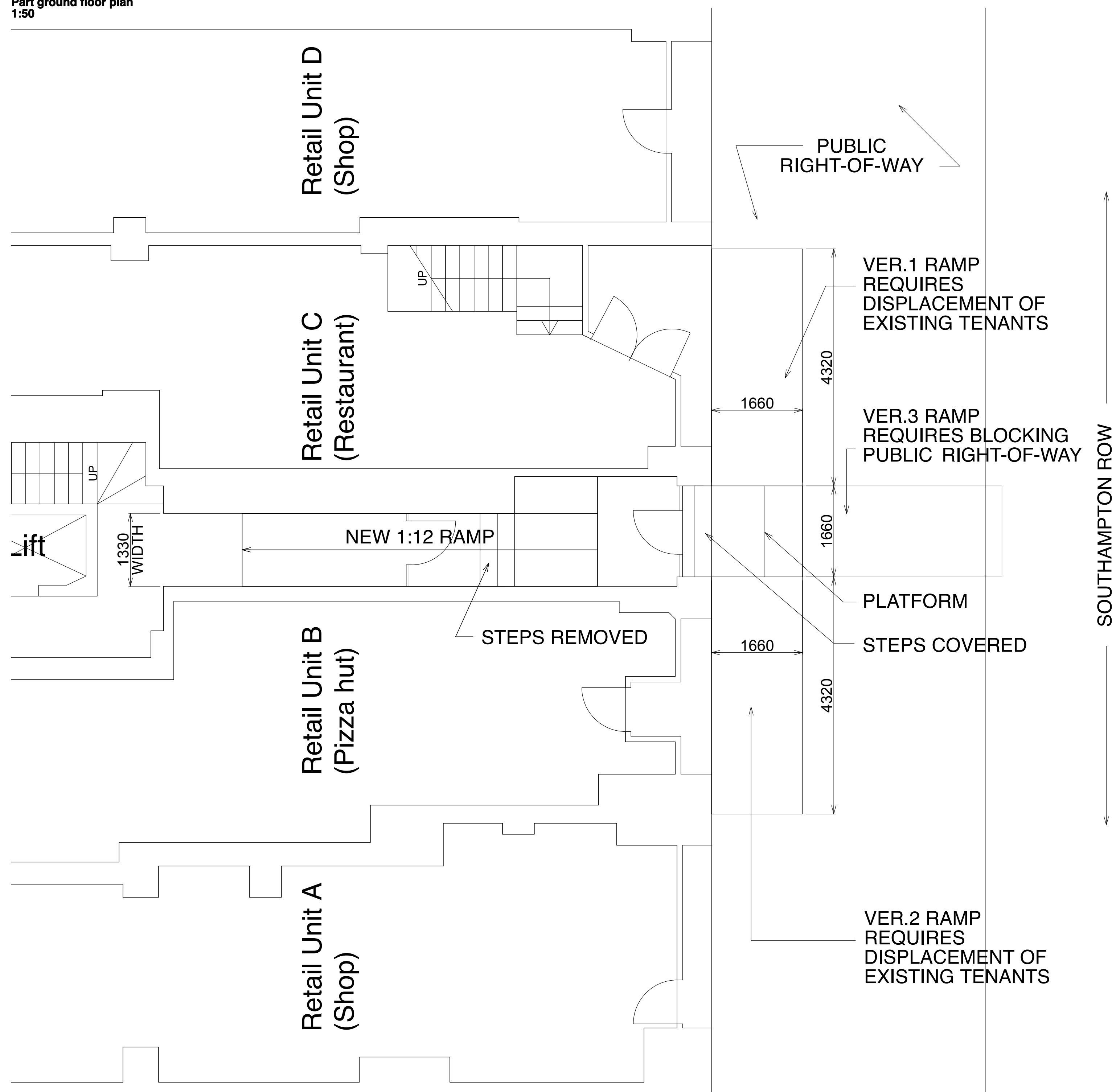
Part ground floor plan 1:50
