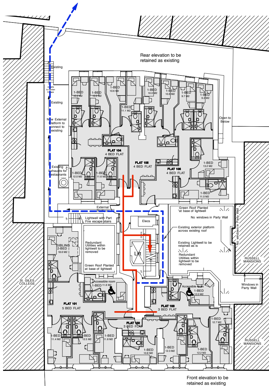
First - Seventh Floor Plans
