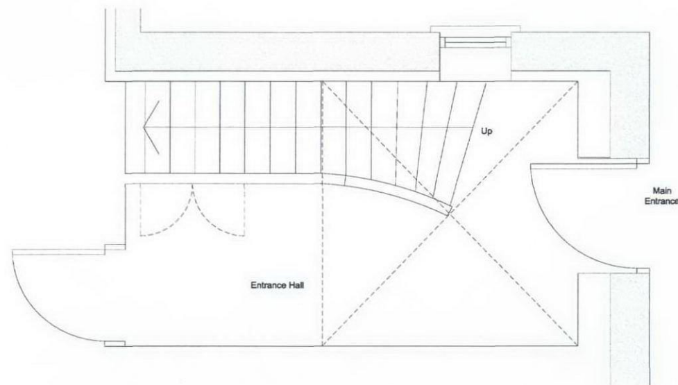
Plan Of Stair
