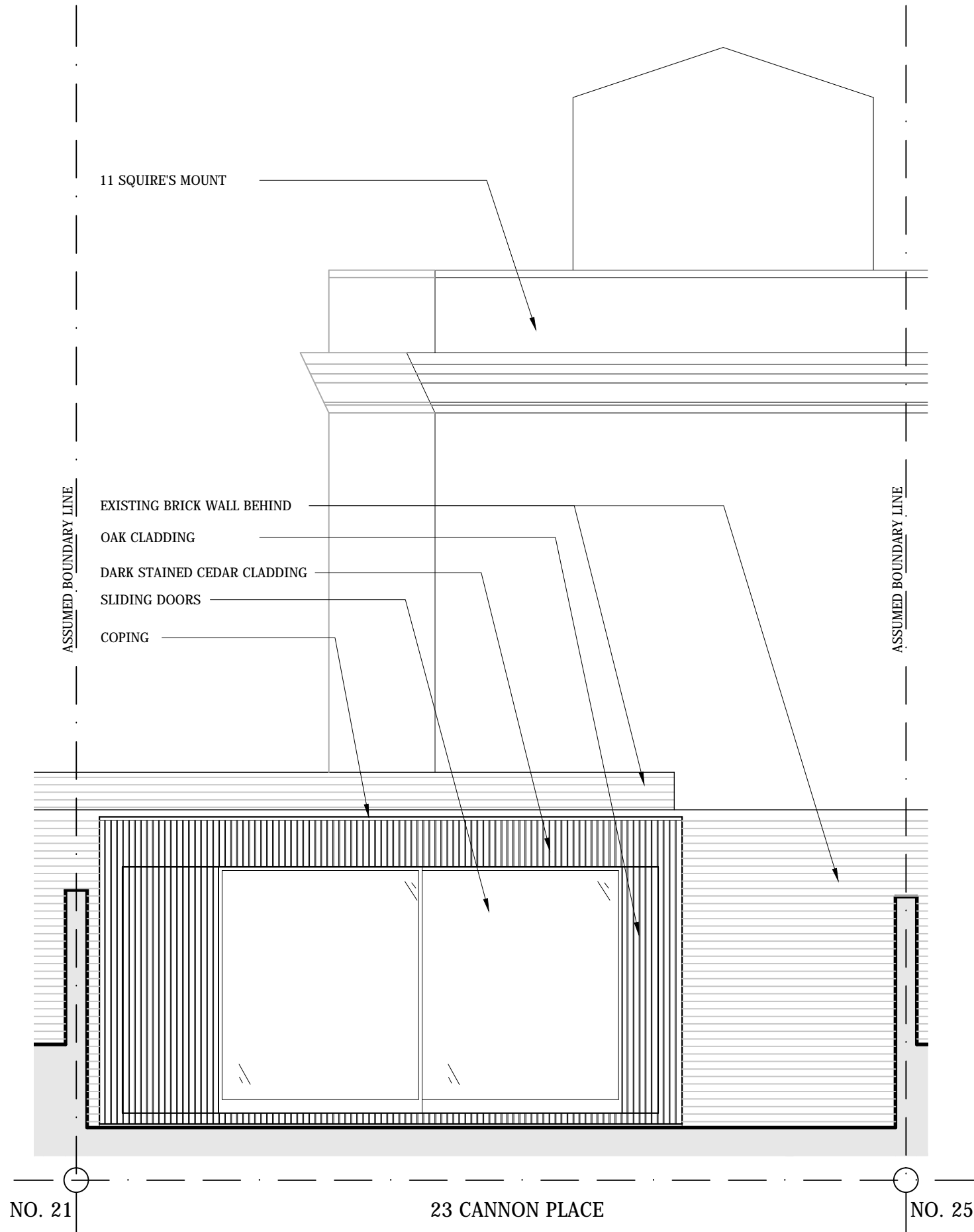
1 1:50 PROPOSED PLAYHOUSE - FRONT ELEVATION
