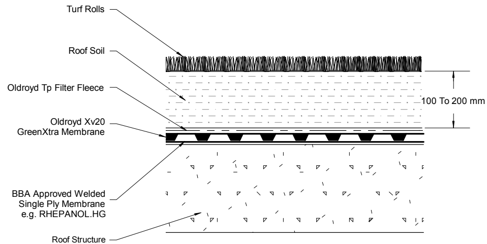
Turfed Roof
