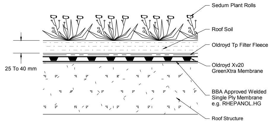
Planted Roof (Sedum or similar)
