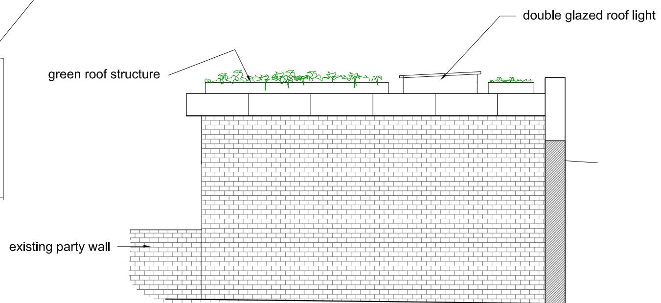
SIDE ELEVATIONS
