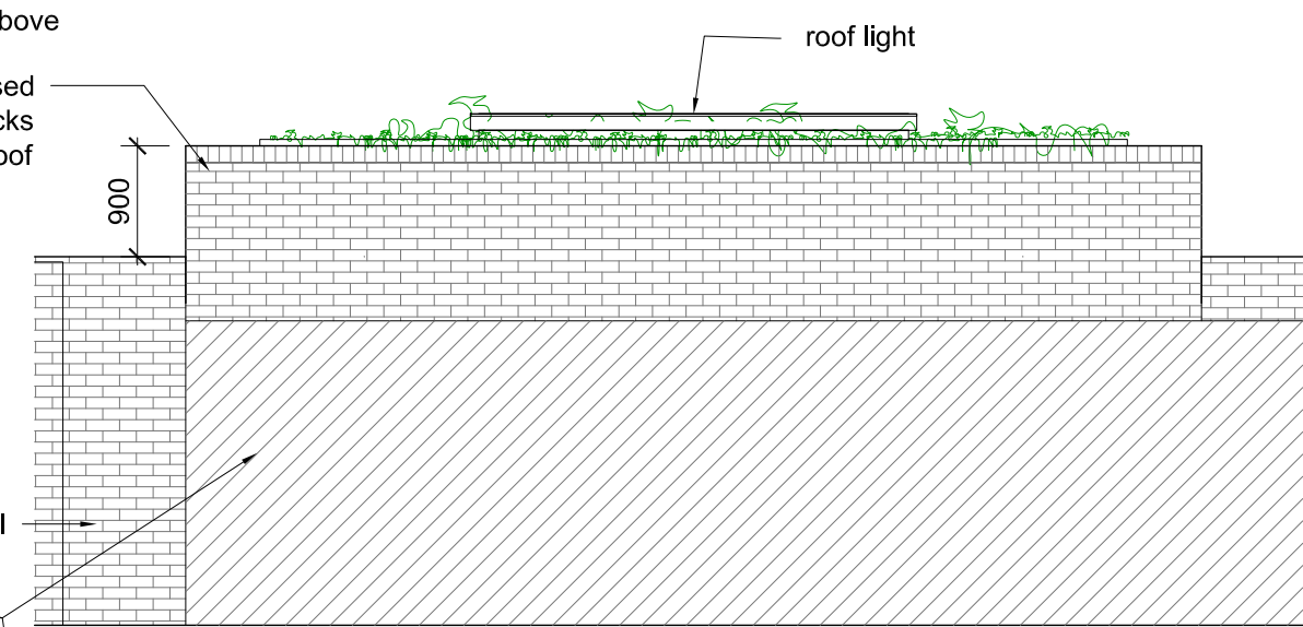
REAR ELEVATION
