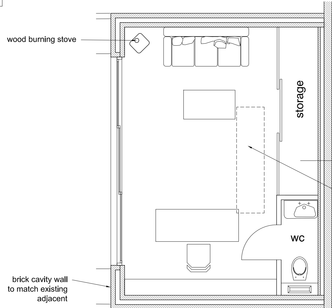
PLAN
