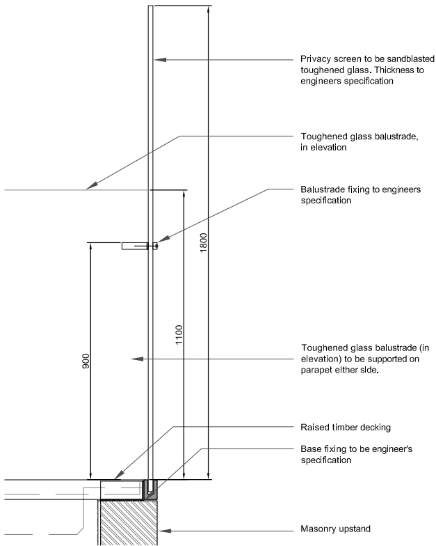
③ Section B Second Floor
