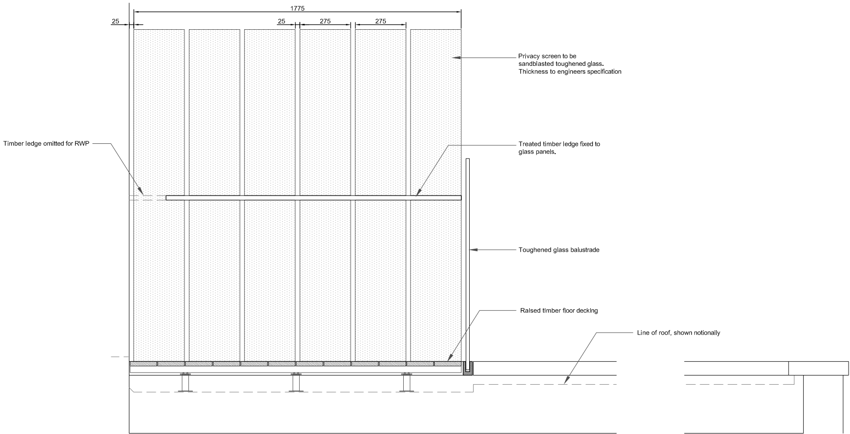
① Elevation Second Floor
