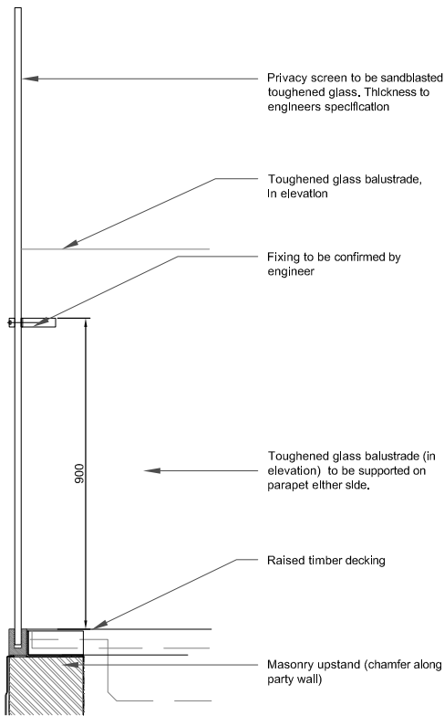
② Section A Second Floor
