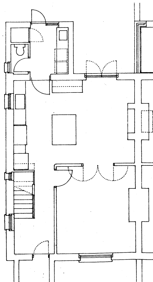
EXISTING LOWER GROUND FLOOR 1:100
