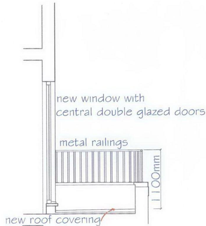
SECTION THROUGH REAR BALCONY (PROPOSED) FIRST FLOOR FLAT AS PROPOSED
