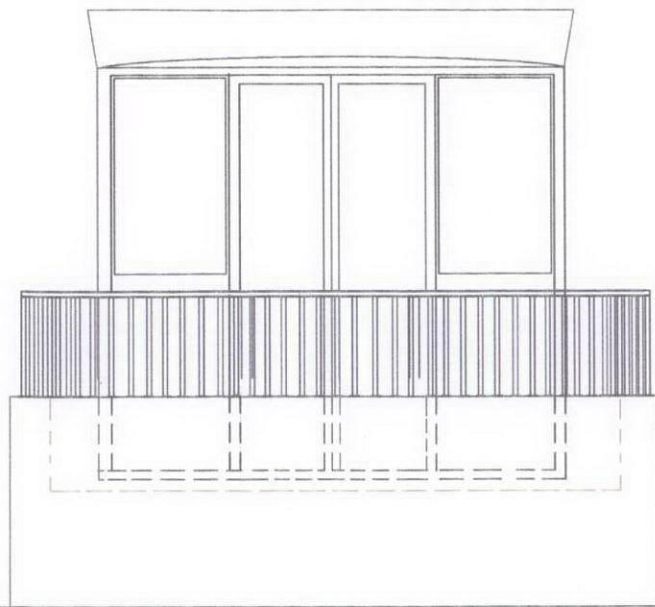
FIRST FLOOR FLAT (REAR) AS PROPOSED PART ELEVATION
