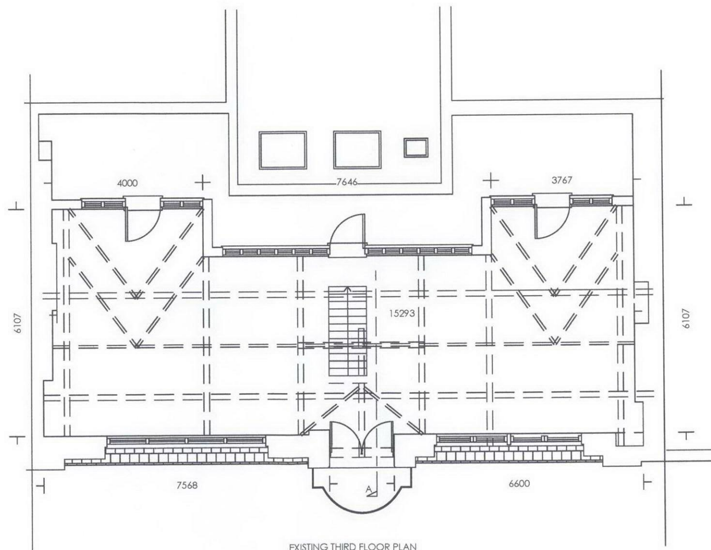
EXISTING THIRD FLOOR PLAN
