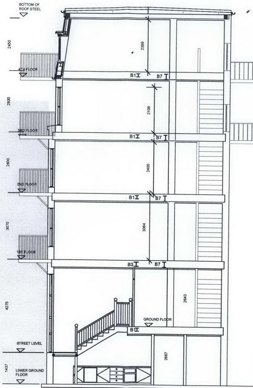
SECTION B-B
