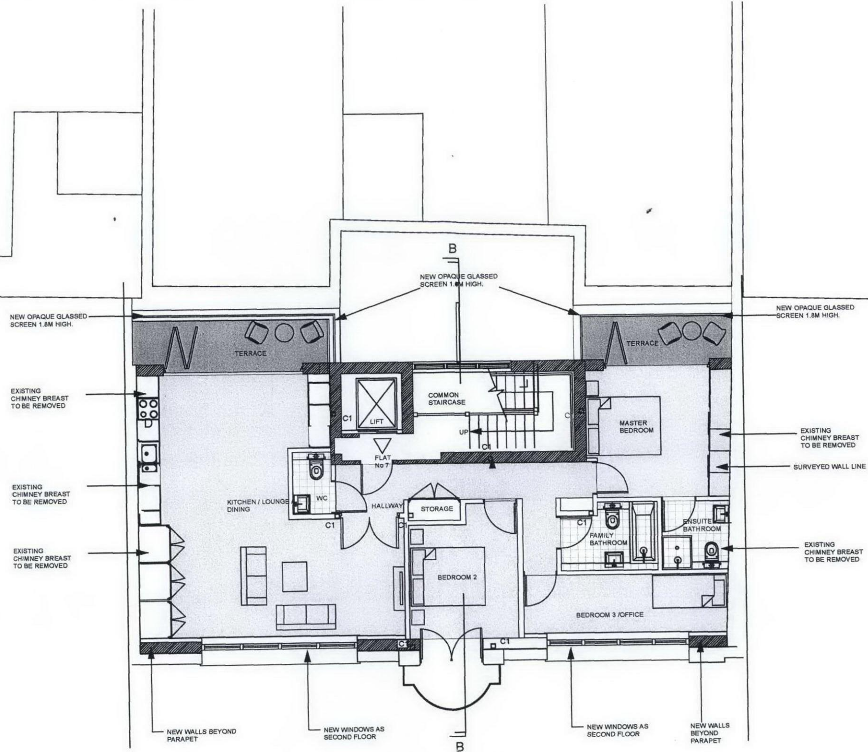
THIRD FLOOR PLAN AREA OF FLAT 7 - 1072 SQ FT
