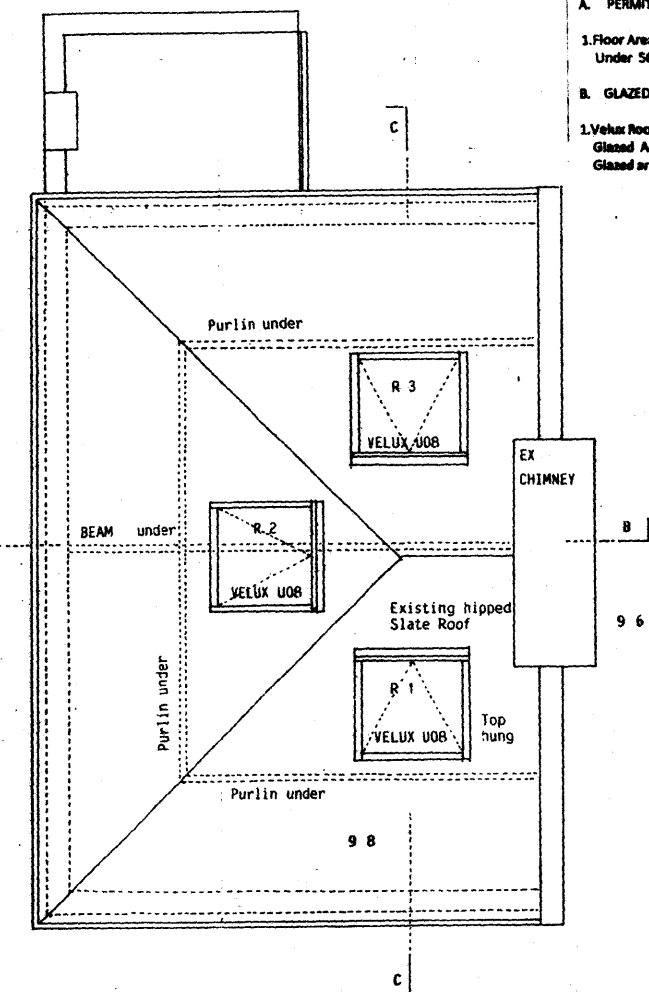
PROPOSED ROOF PLAN 1:100 (including New Rooflights)
