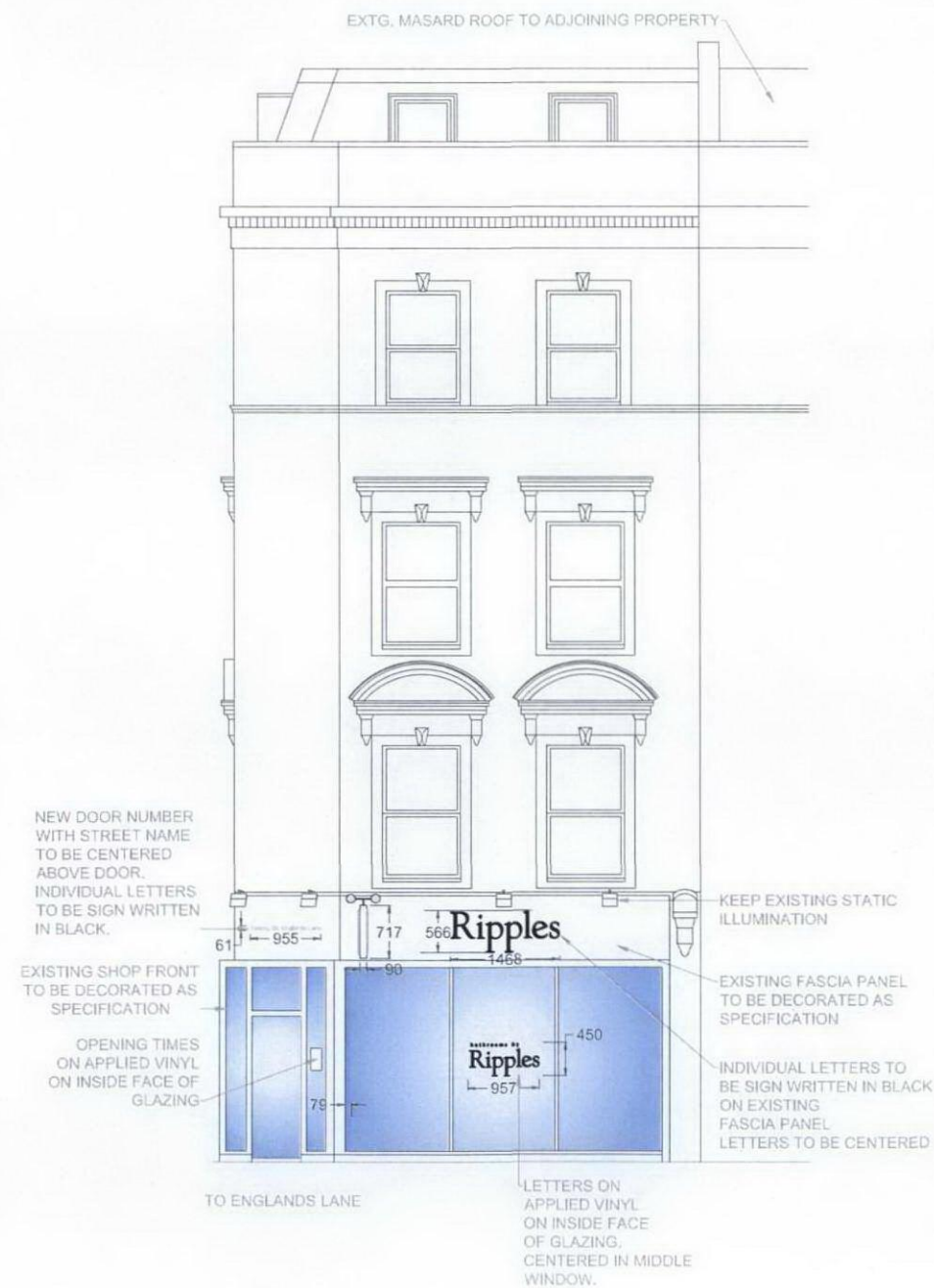
PROPOSED 1:50 FRONT ELEVATION
