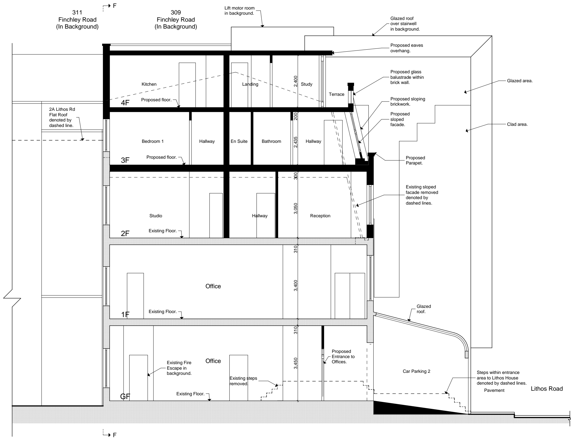
Proposed Section C-C / West Elevation
