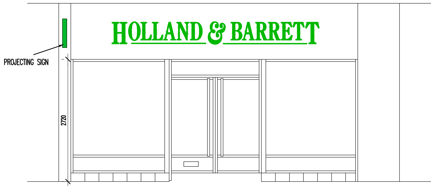
EXISTING SHOP FRONT ELEVATION 1:50 @ A1
