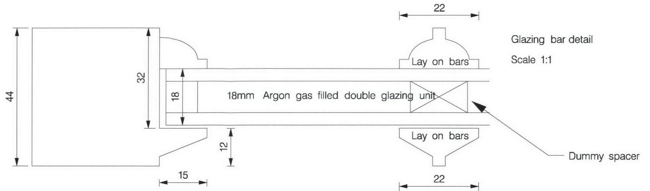
Stile & head rail detail Scale 1:1
