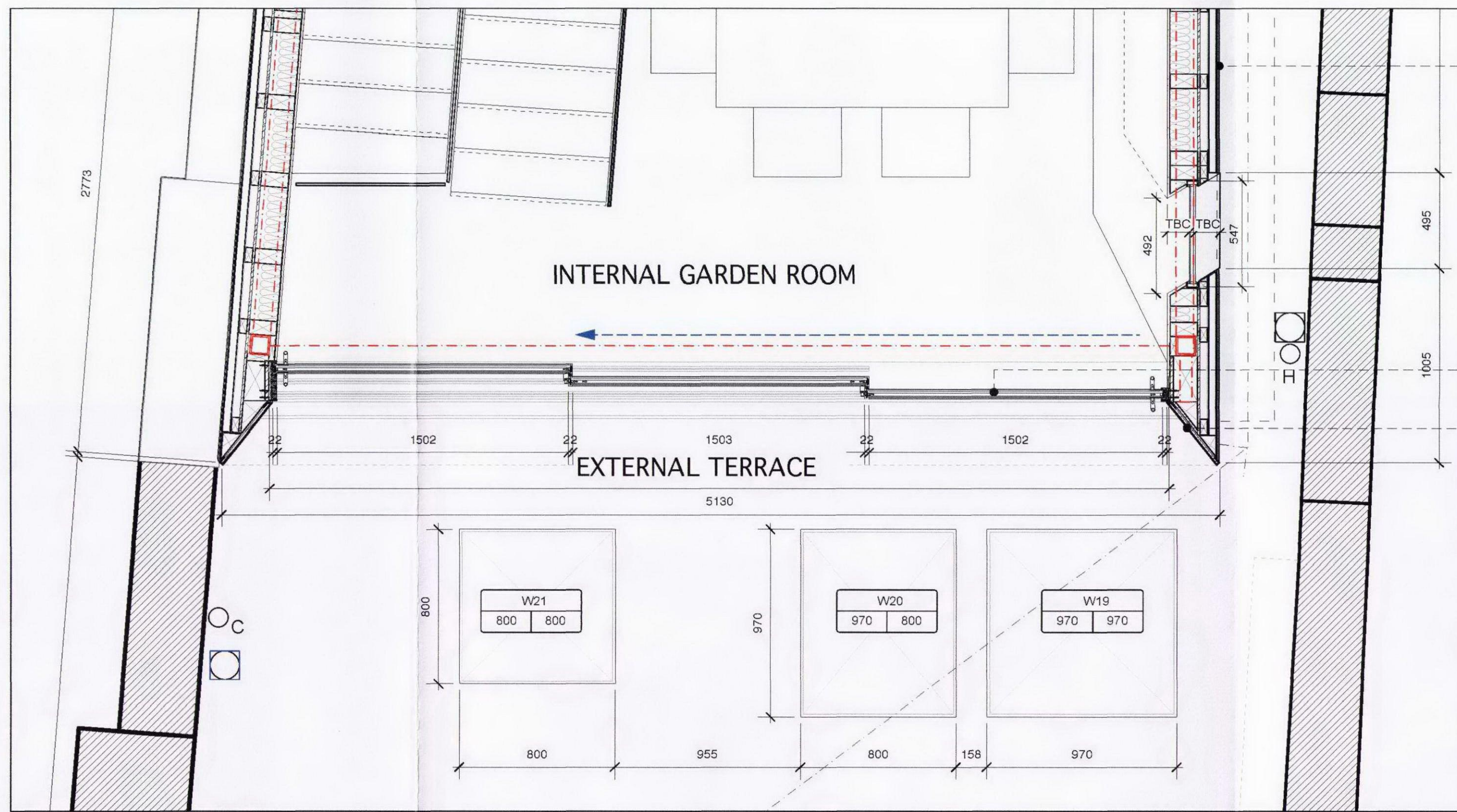
02 GARDEN ROOM PLAN - THRESHOLD DETAIL 1:20 @ A0
