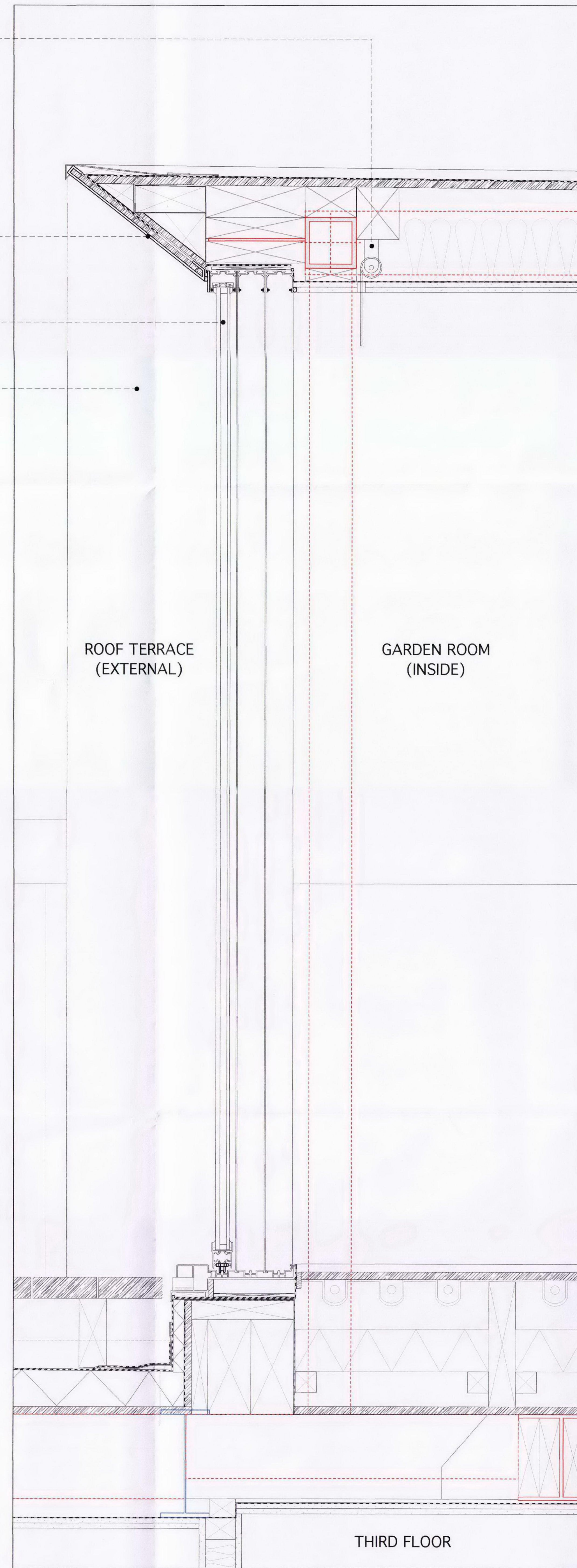
04 GARDEN ROOM - THRESHOLD DETAIL 1:5 @ A0
