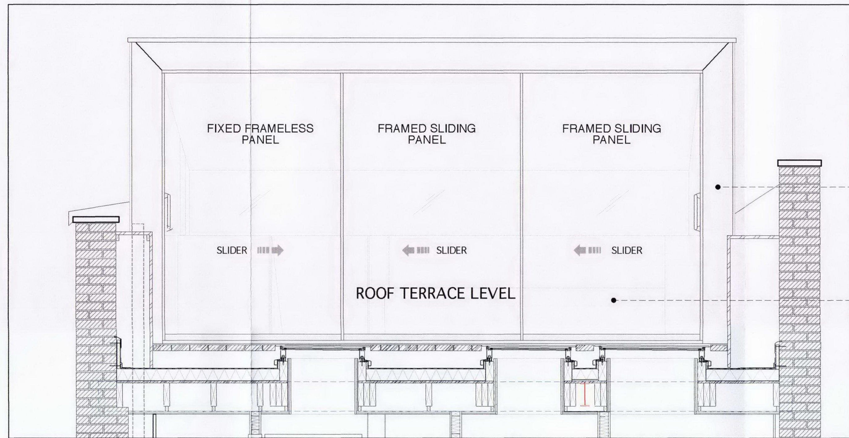
03 GARDEN ROOM ELEVATION 1:20 @ A0
