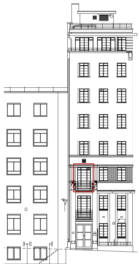
Window Location D John Street Elevation Scale NTS
