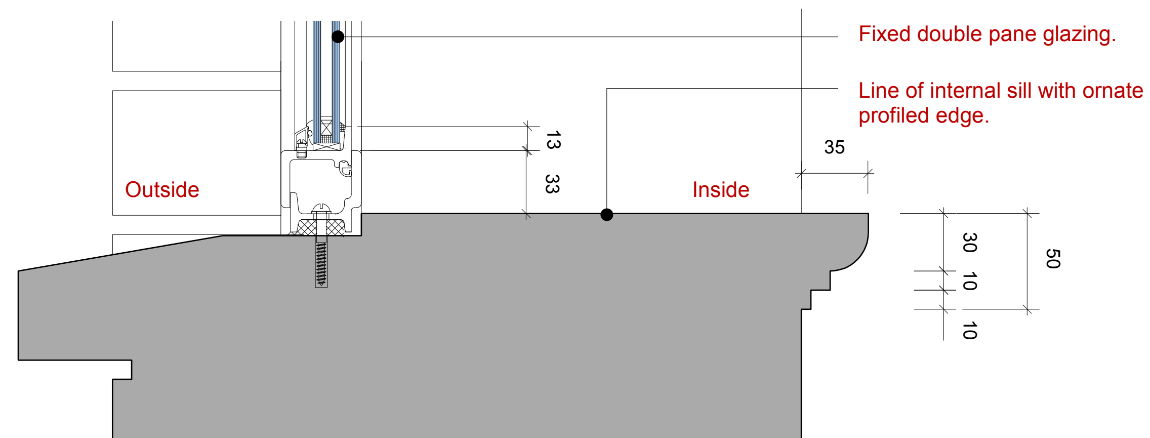
Detail C - Section Scale 1:2 @ A1
