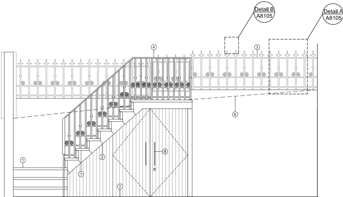
Elevation Door Closed
