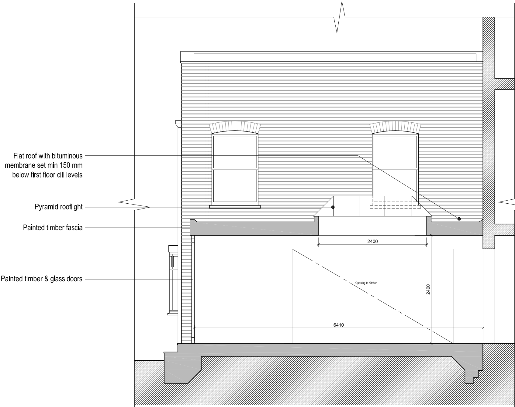
SECTION D-D OF PROPOSED EXTENSION
