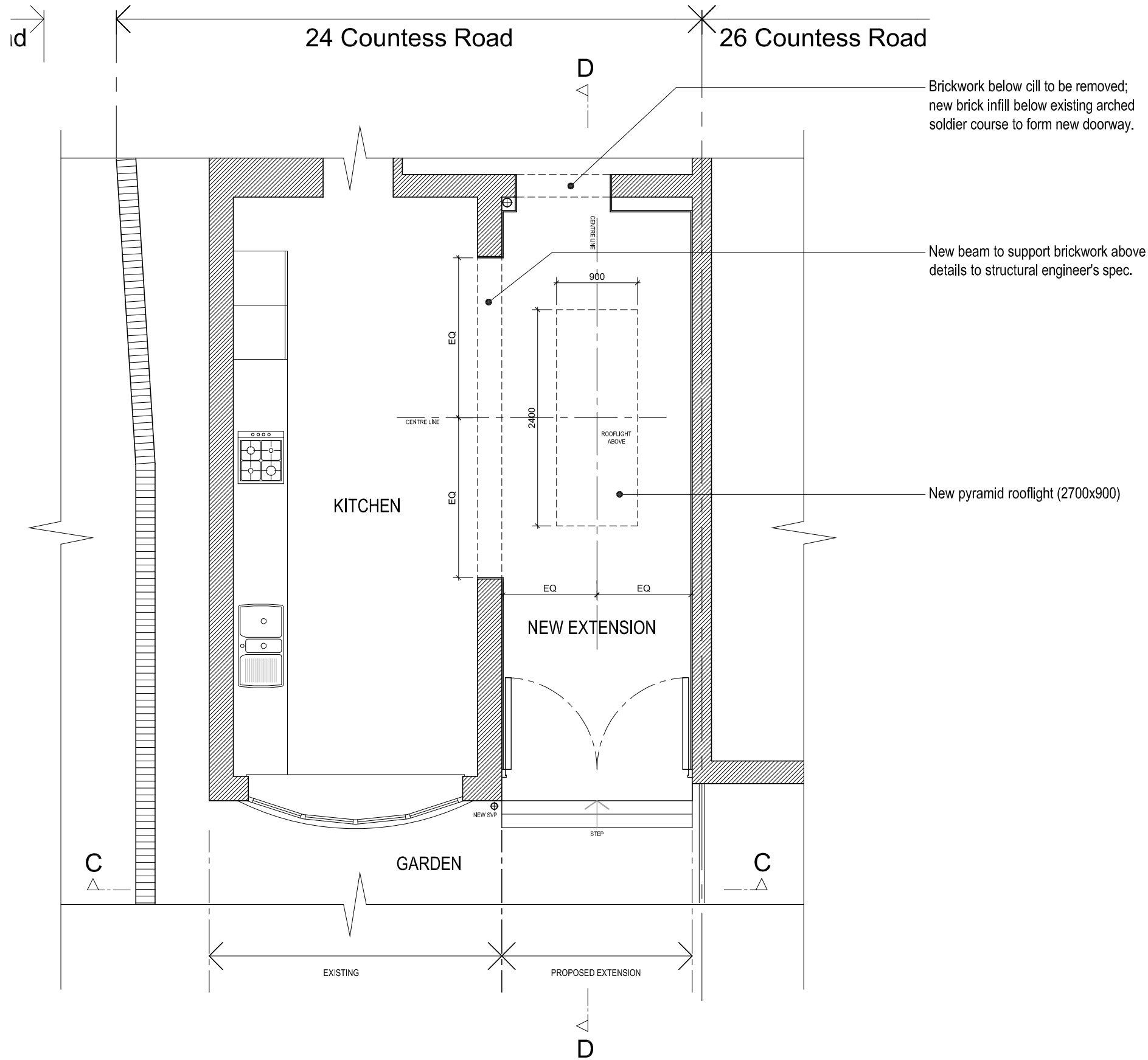
PROPOSED GROUND FLOOR PLAN (REAR)
