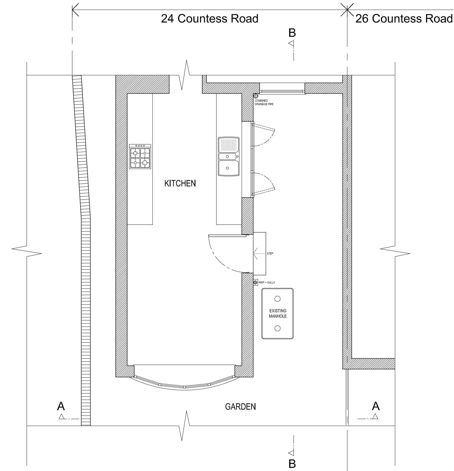
EXISTING GROUND FLOOR PLAN (REAR)
