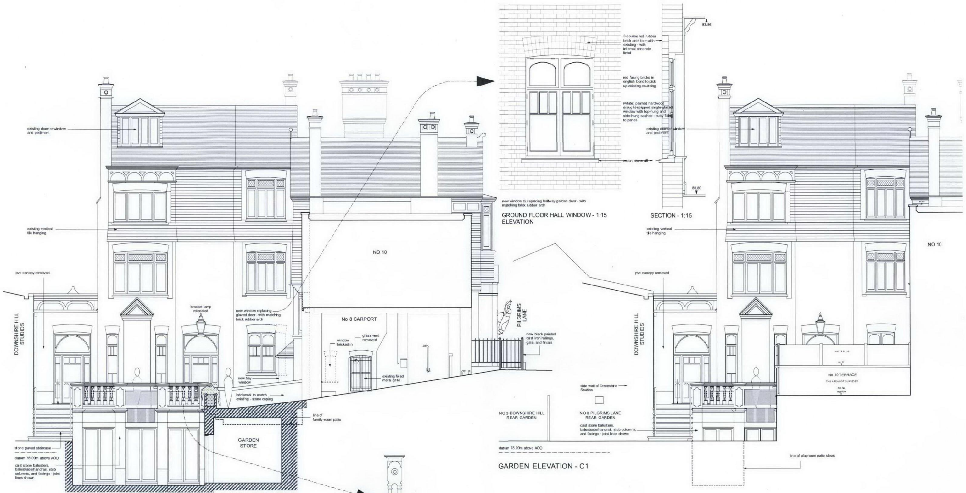
ELEVATION C
