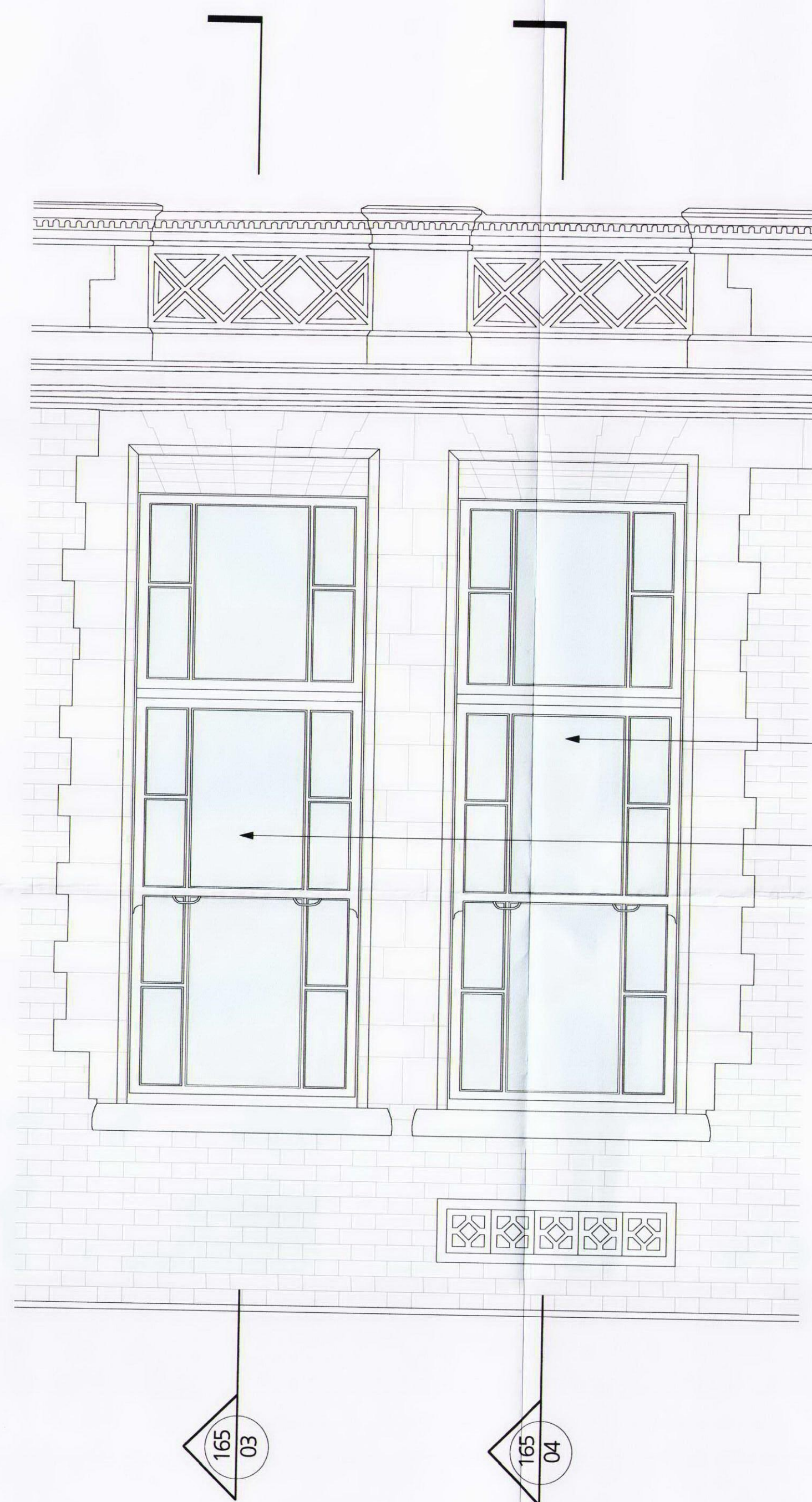
01 Proposed Windows Typical External Elevation 1:20 @ A1
