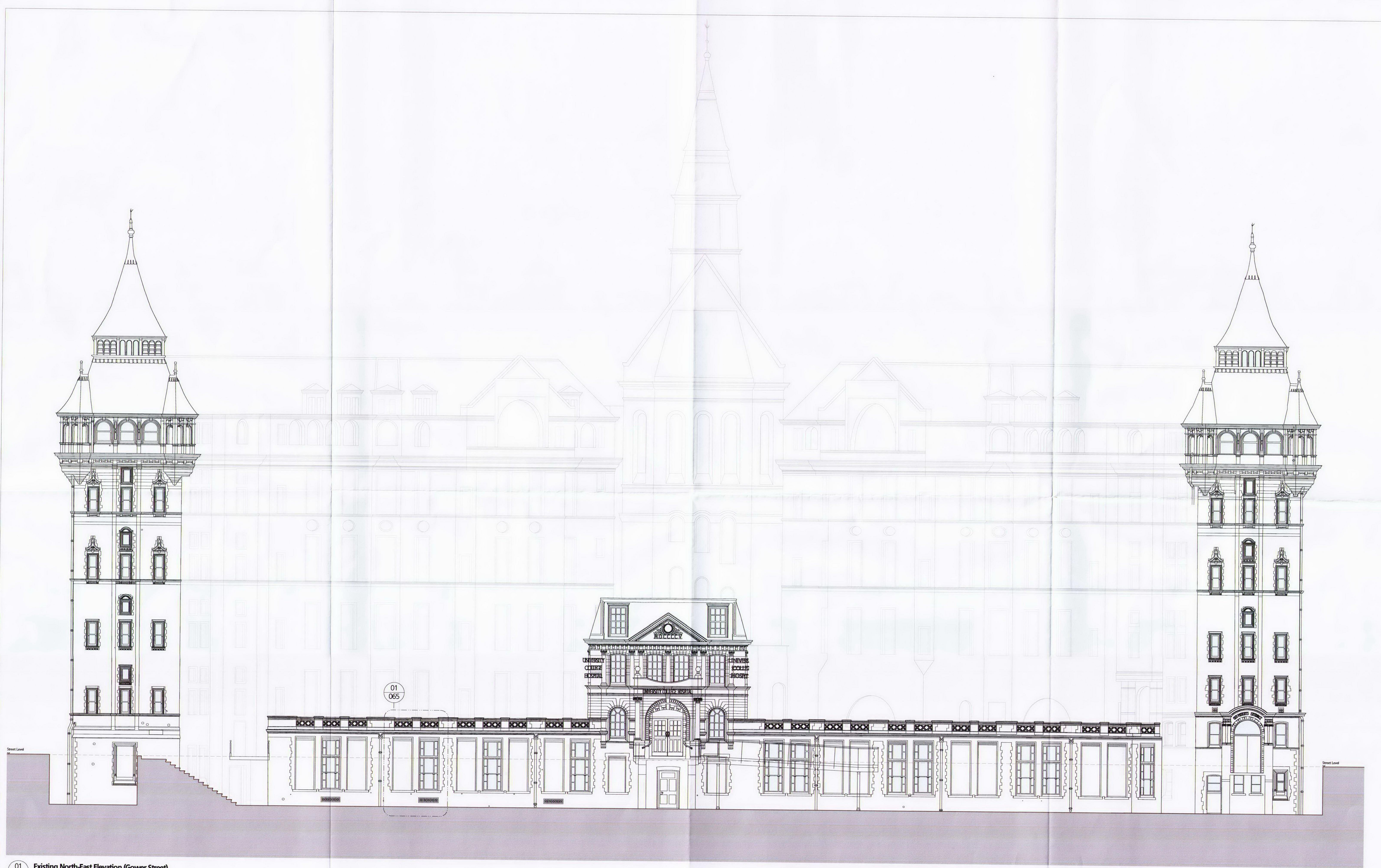
01 Existing North-East Elevation (Gower Street) 1:100 @ A1, 1:200 @ A3
