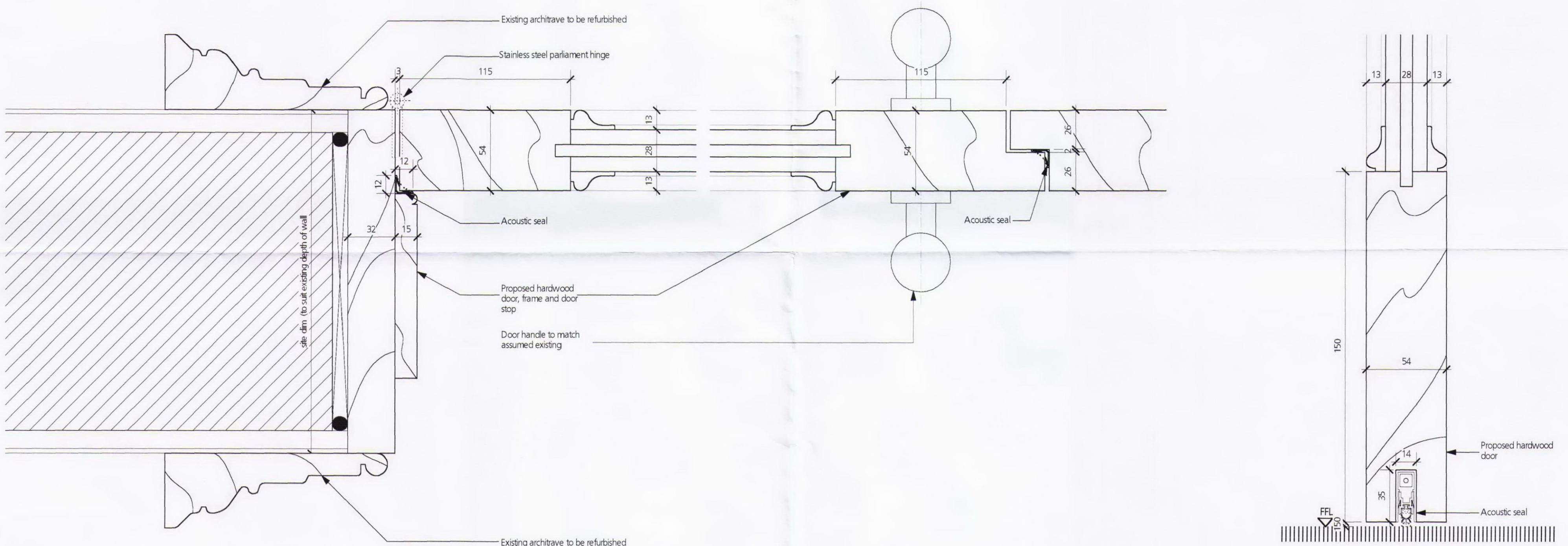
02 Jamb Detail showing acoustic seals - 1:2
