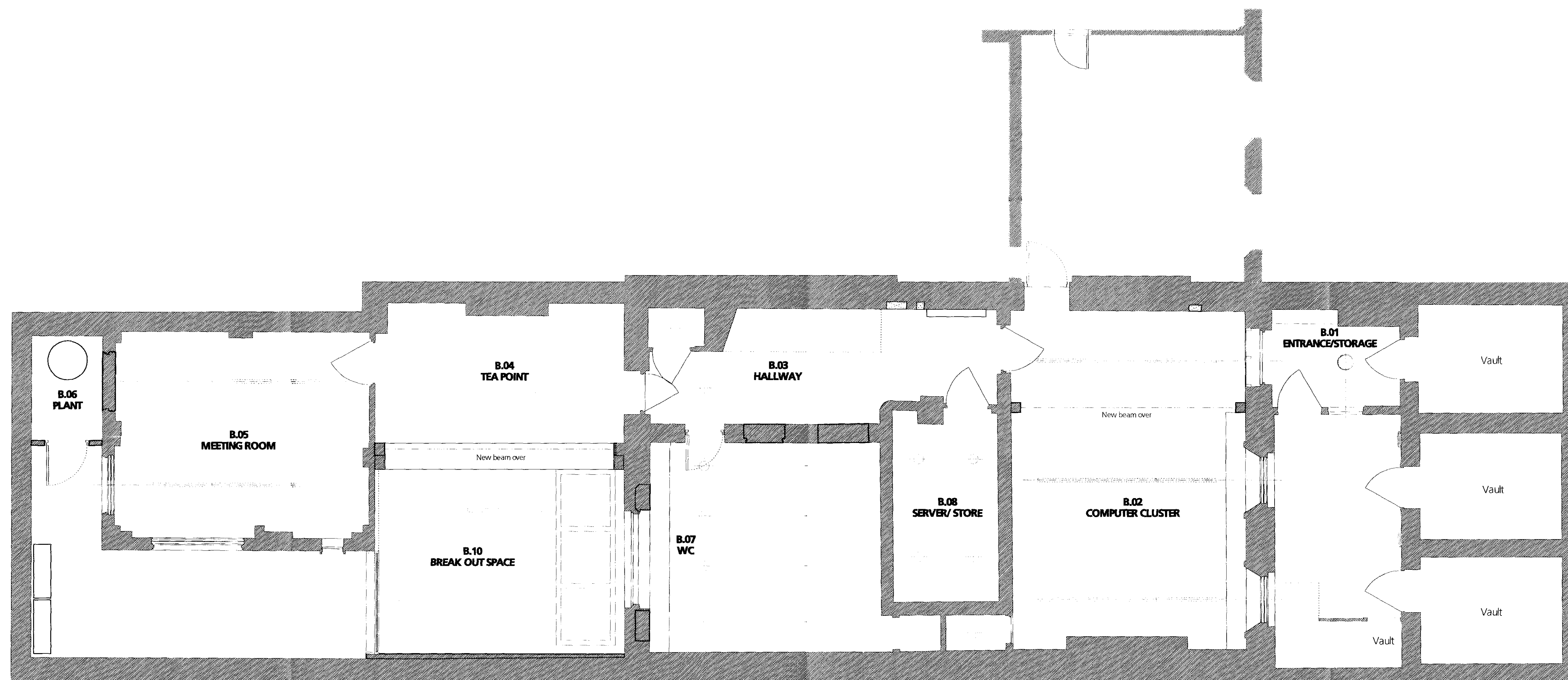
1 Lower Ground Floor Reflected Ceiling Plan 1:100 @ A3 & 1:50 @ A1
