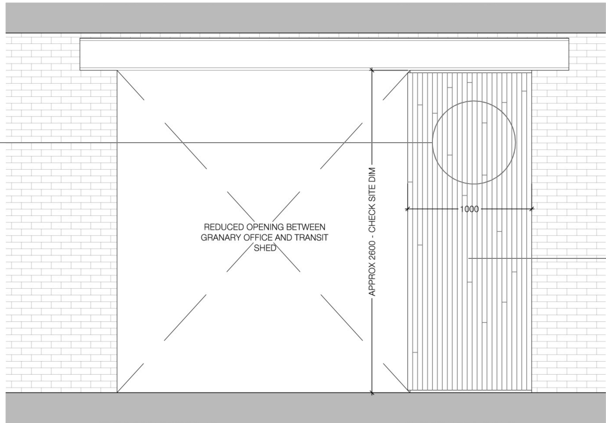
New timber wall extension within existing opening
