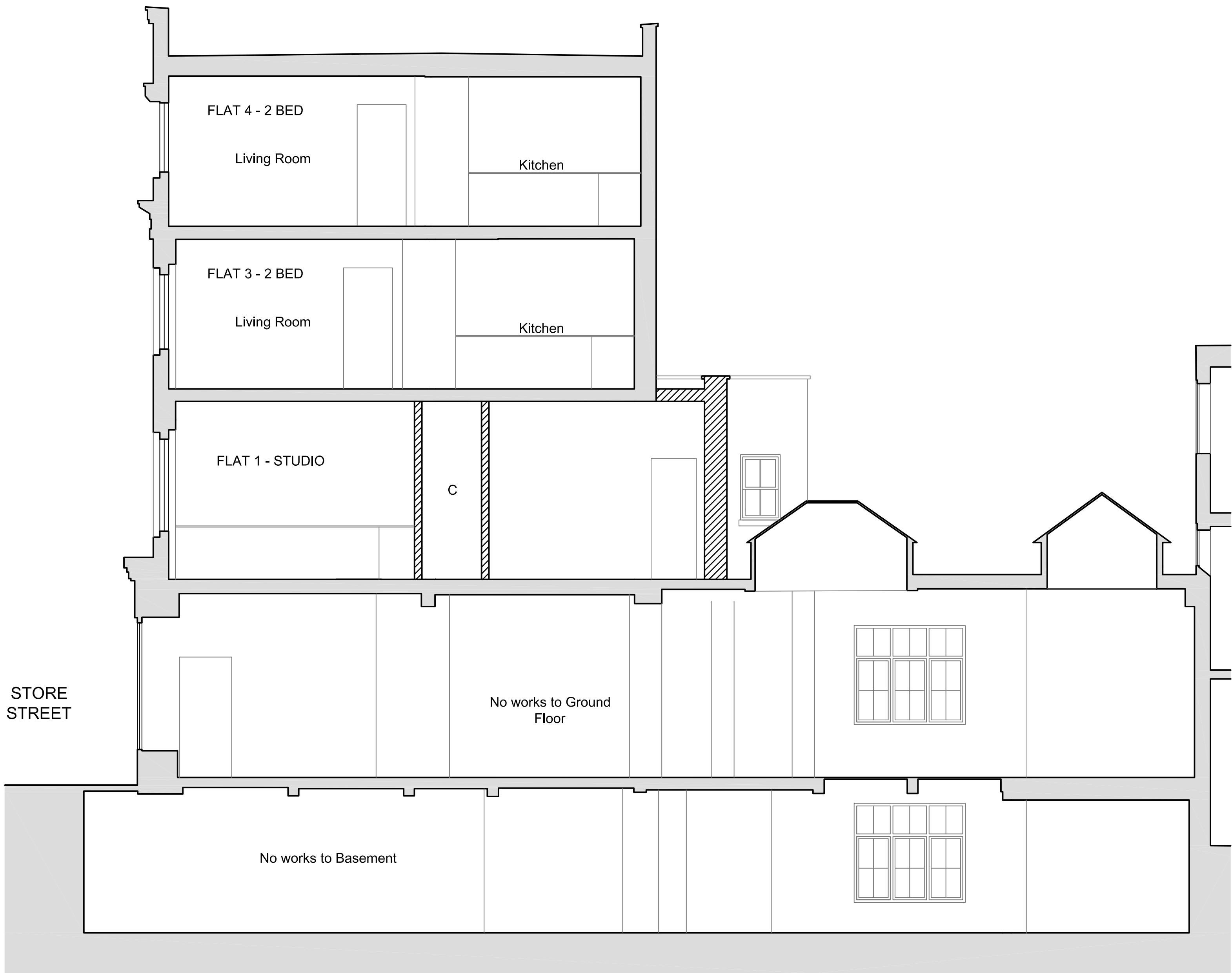
01 (01)800 SECTION A-A As Proposed
