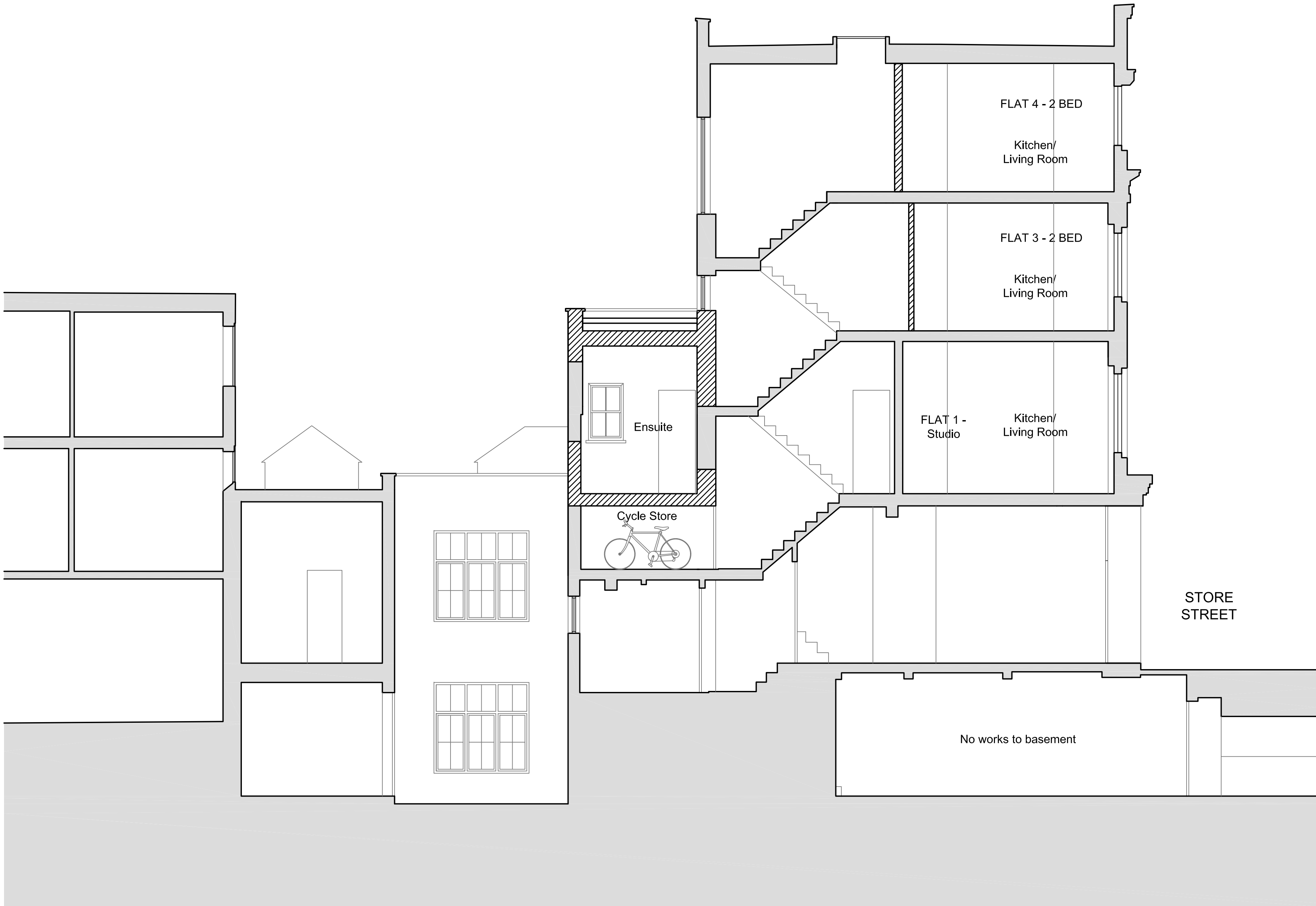
01 (01)801 SECTION B-B As Proposed
