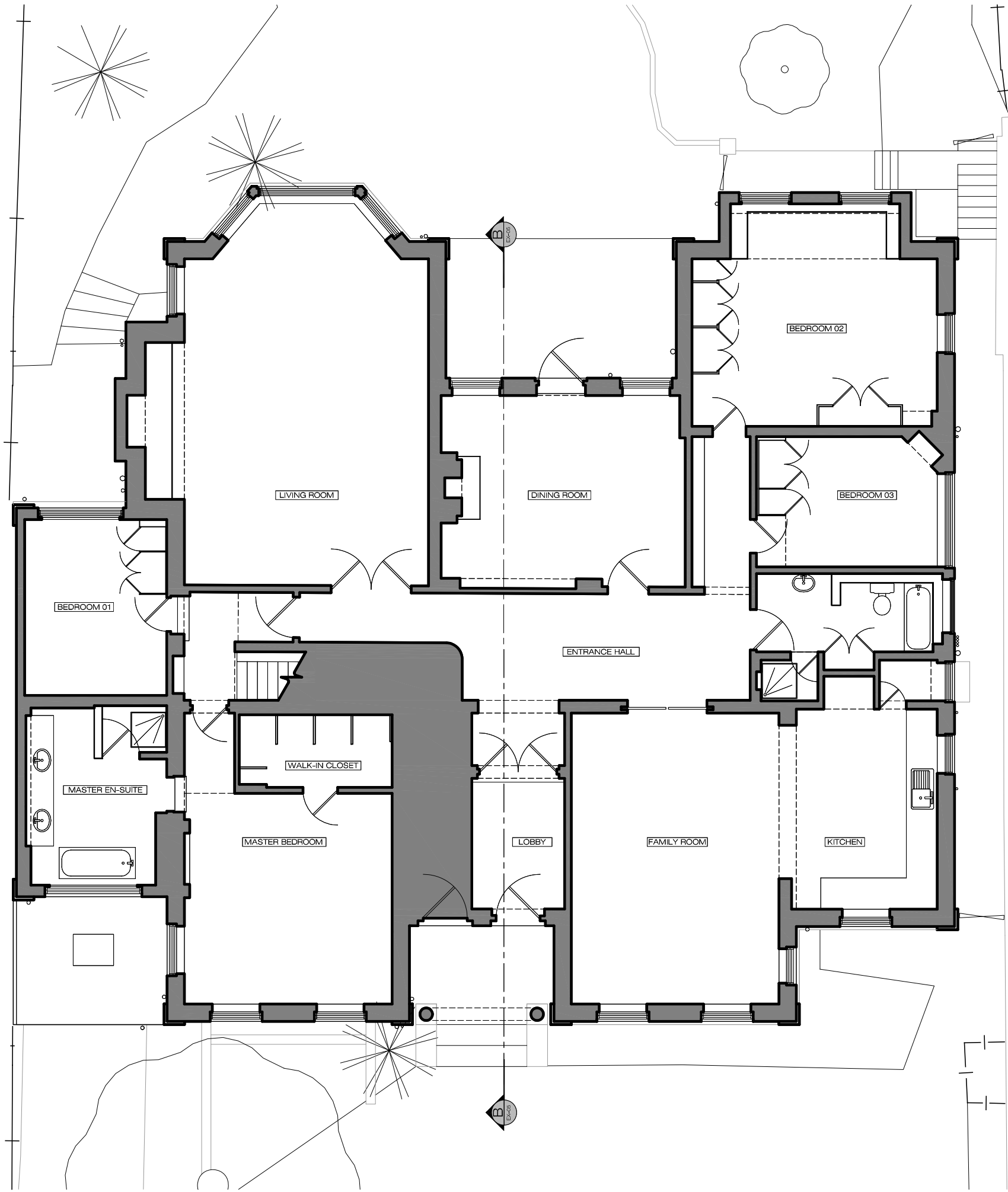
EXISTING GROUND FLOOR PLAN SCALE 1:50@A1 EX-02
